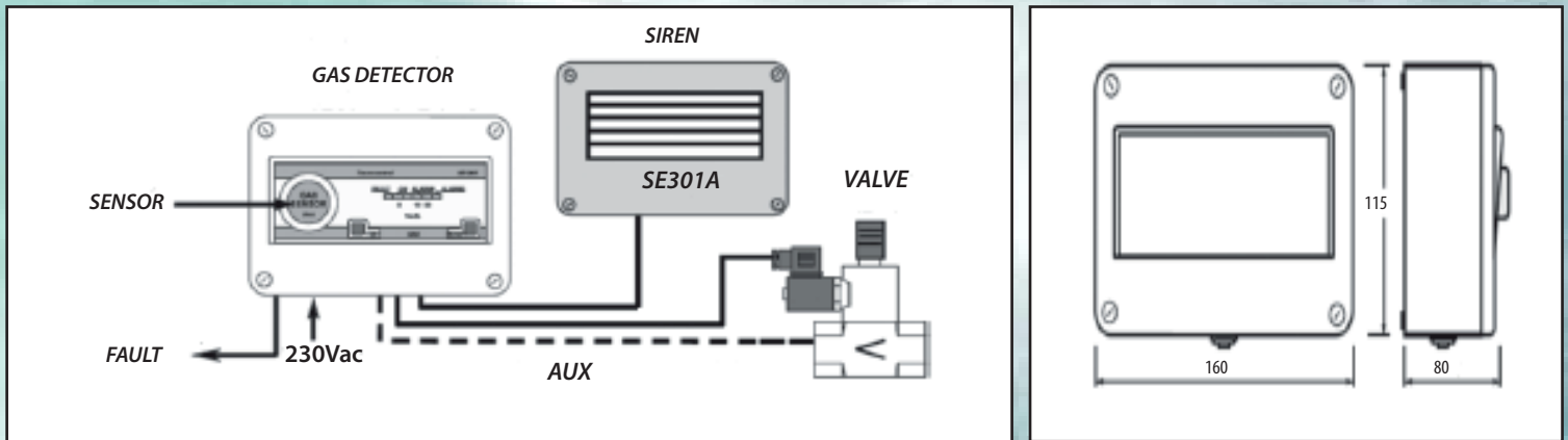
Example of SE 126K installation diagram with solenoid valve and siren.
